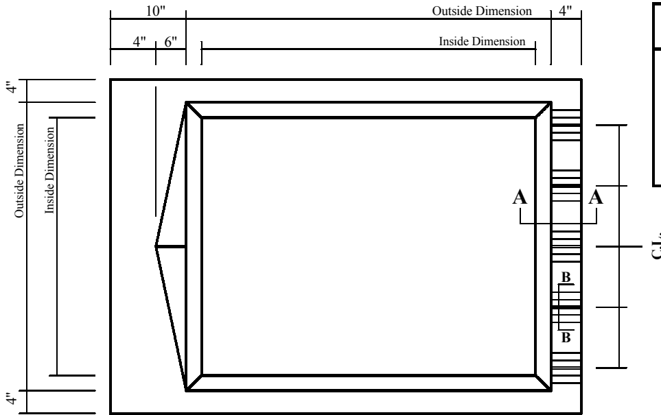
PLAN VIEW
