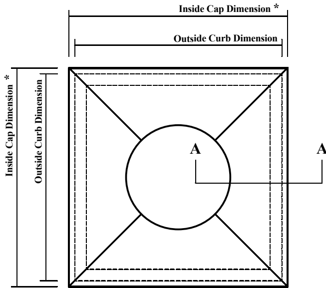
PLAN VIEW
